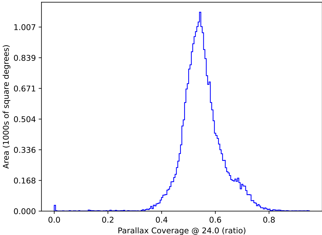
too_elab_r16_d3_griz_v3.4_10yrs : Parallax Coverage @ 24.0
