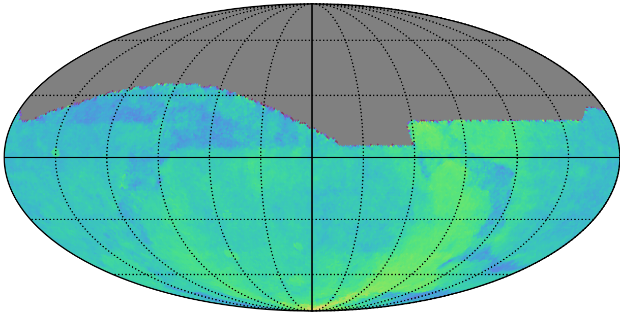
too_elab_r16_d3_griz_v3.4_10yrs : Parallax Coverage @ 22.4
