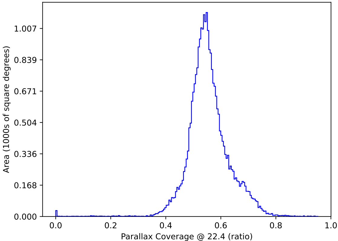
too_elab_r16_d3_griz_v3.4_10yrs : Parallax Coverage @ 22.4
