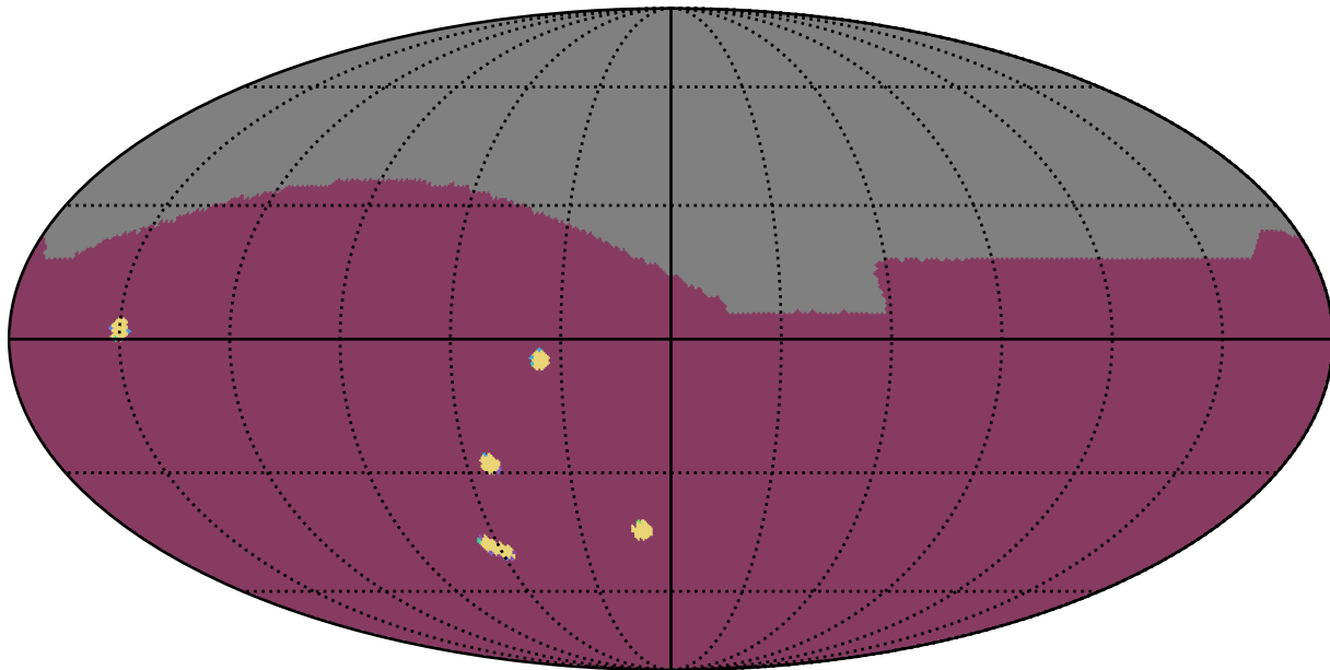
too_elab_r16_d3_griz_v3.4_10yrs : NumberOfQuickRevisits
