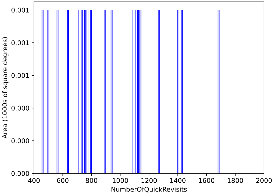
too_elab_r16_d3_griz_v3.4_10yrs : NumberOfQuickRevisits
