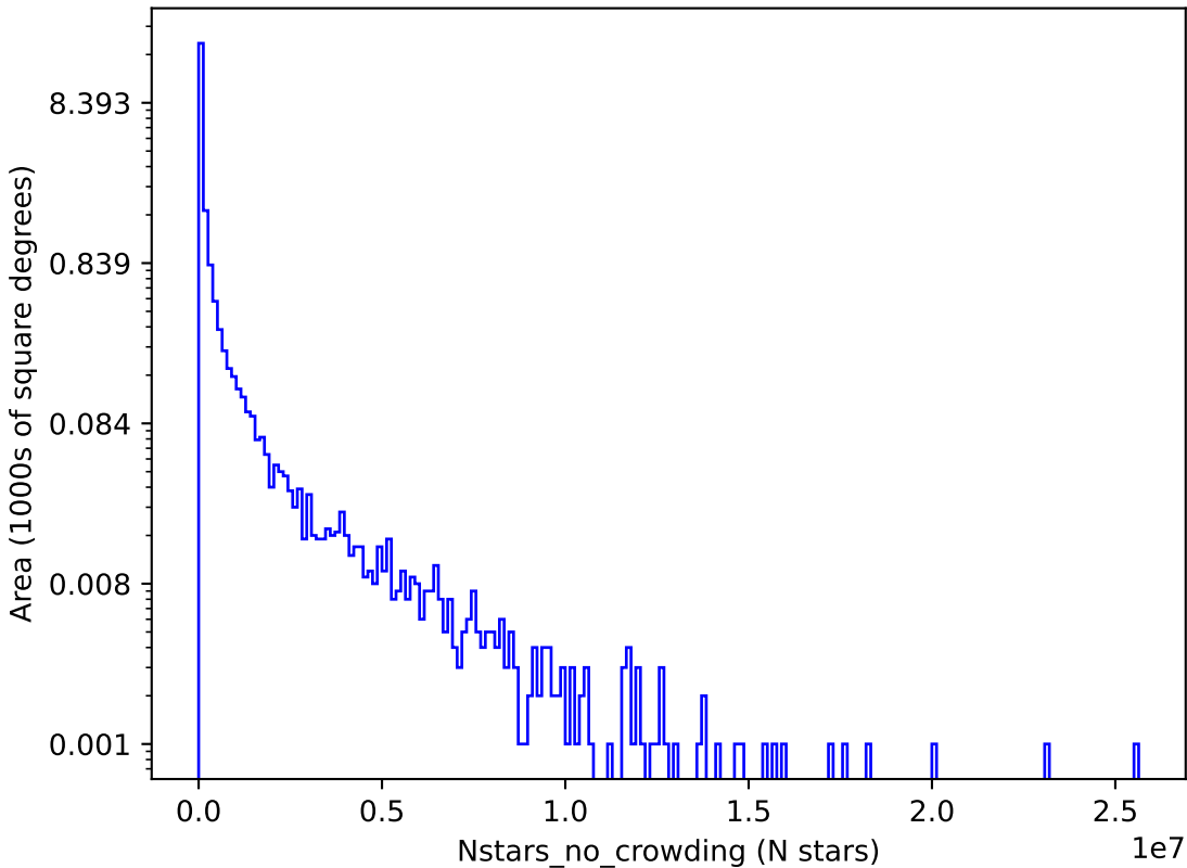
too_elab_r16_d3_griz_v3.4_10yrs y: Nstars_no_crowding
