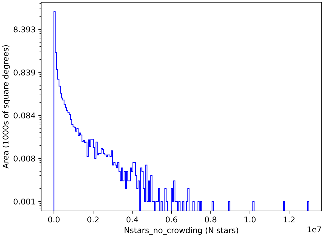
too_elab_r16_d3_griz_v3.4_10yrs g: Nstars_no_crowding
