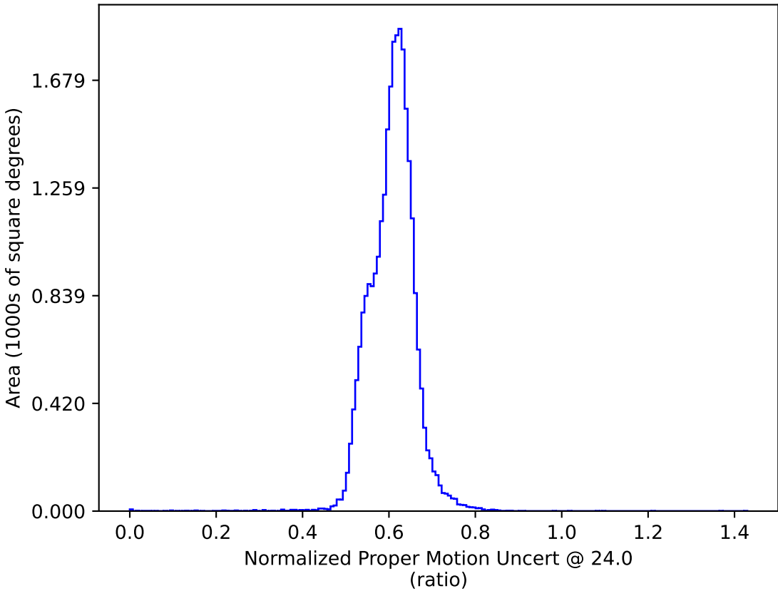
too_elab_r16_d3_griz_v3.4_10yrs : Normalized Proper Motion Uncert @ 24.0
