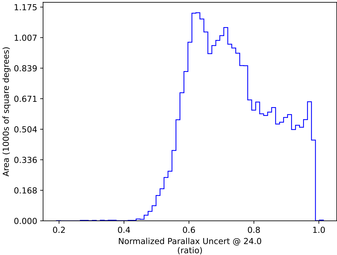
too_elab_r16_d3_griz_v3.4_10yrs : Normalized Parallax Uncert @ 24.0
