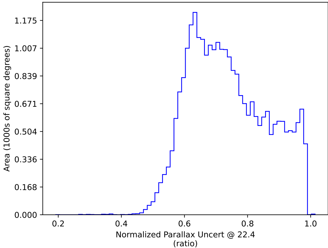
too_elab_r16_d3_griz_v3.4_10yrs : Normalized Parallax Uncert @ 22.4
