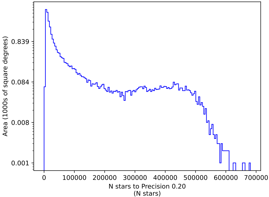
too_elab_r16_d3_griz_v3.4_10yrs r: N stars to Precision 0.20
