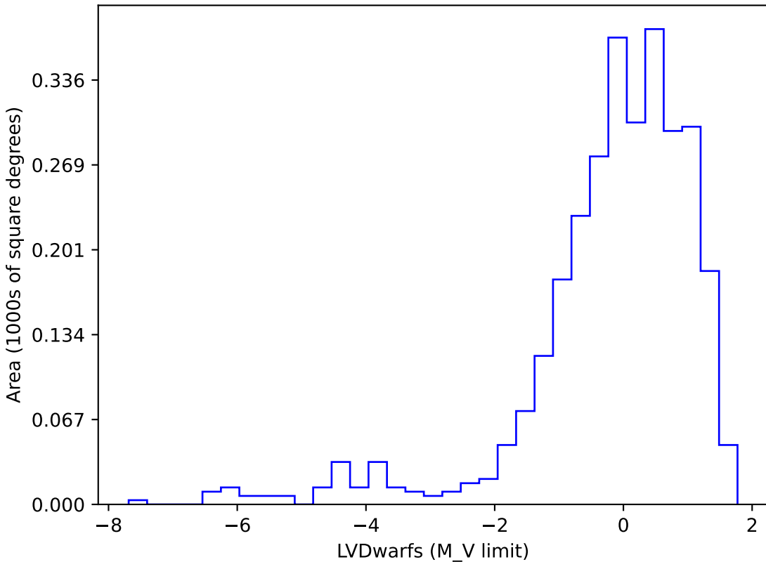
too_elab_r16_d3_griz_v3.4_10yrs gi SCP: LVDwarfs
