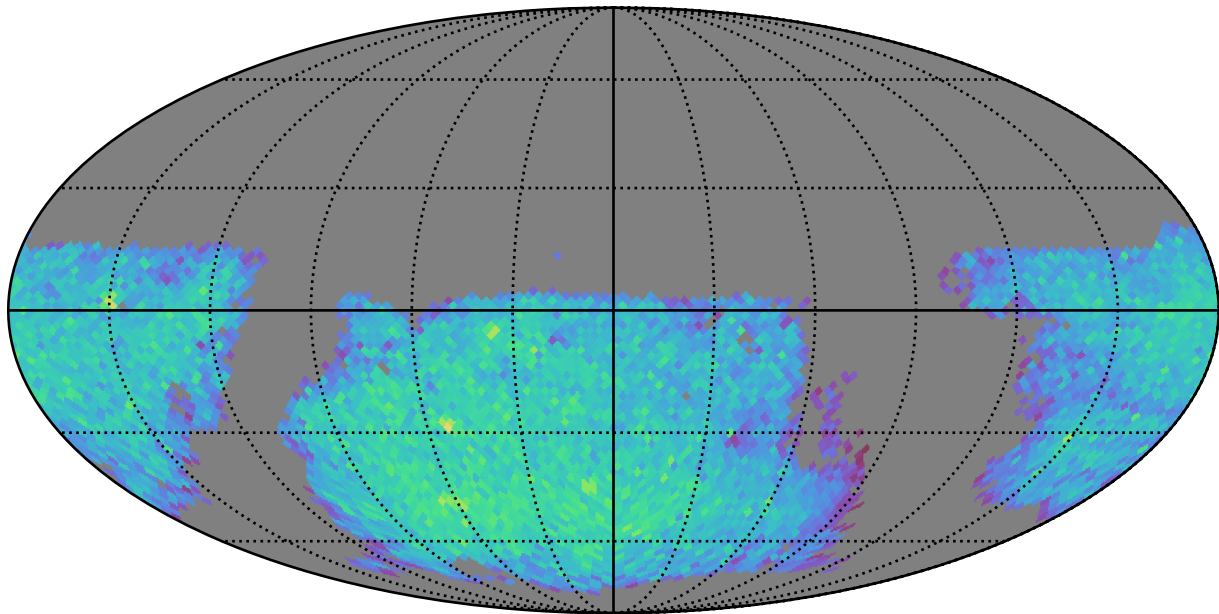
too_elab_r16_d3_griz_v3.4_10yrs gi: LVDwarfs
