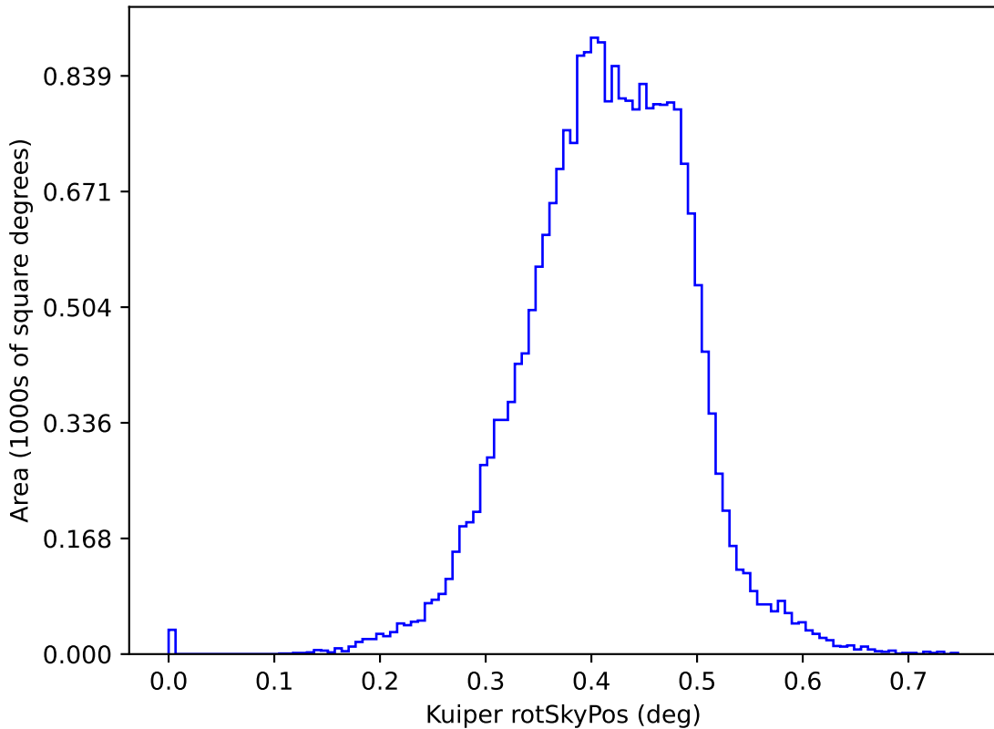
too_elab_r16_d3_griz_v3.4_10yrs y: Kuiper rotSkyPos
