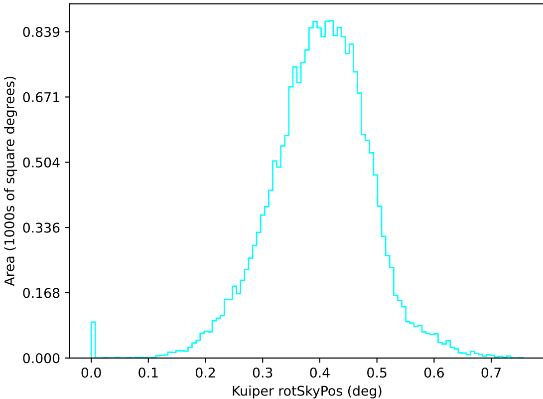
too_elab_r16_d3_griz_v3.4_10yrs u: Kuiper rotSkyPos
