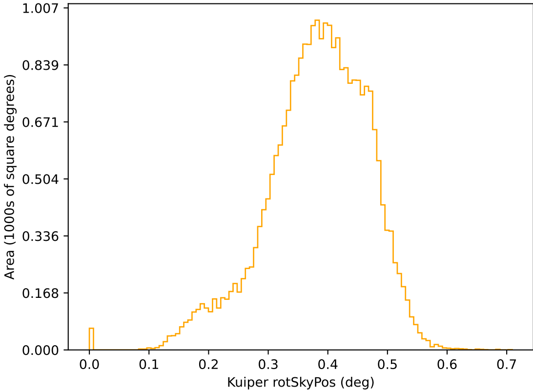
too_elab_r16_d3_griz_v3.4_10yrs r: Kuiper rotSkyPos
