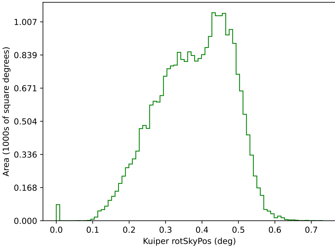
too_elab_r16_d3_griz_v3.4_10yrs g: Kuiper rotSkyPos
