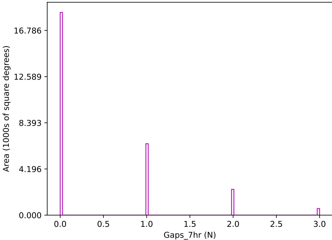
too_elab_r16_d3_griz_v3.4_10yrs z band: Gaps_7hr
