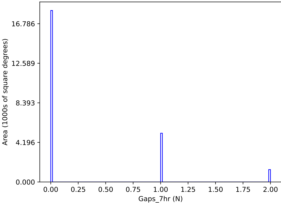
too_elab_r16_d3_griz_v3.4_10yrs y band: Gaps_7hr
