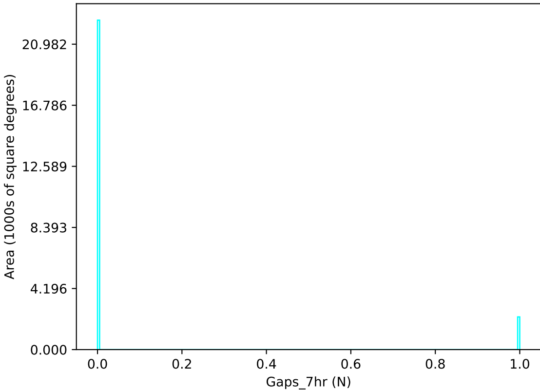
too_elab_r16_d3_griz_v3.4_10yrs u band: Gaps_7hr
