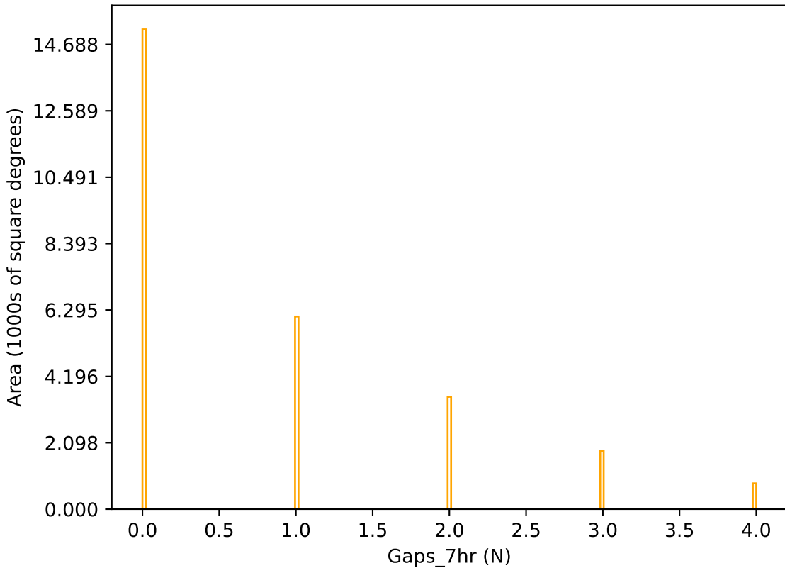
too_elab_r16_d3_griz_v3.4_10yrs r band: Gaps_7hr
