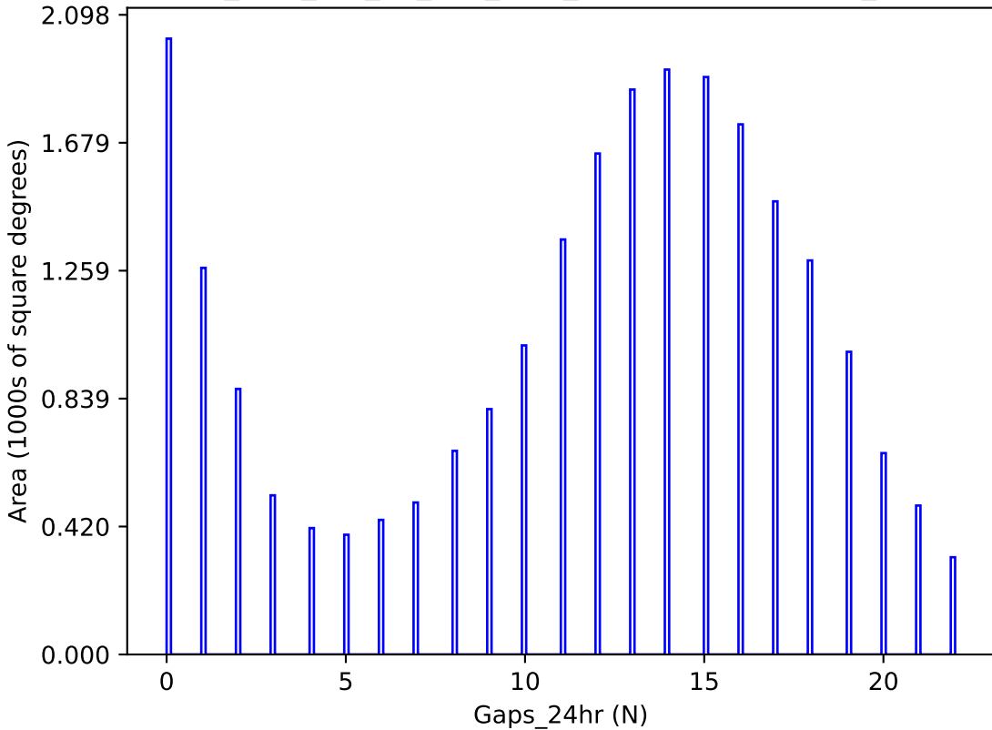
too_elab_r16_d3_griz_v3.4_10yrs y band: Gaps_24hr
