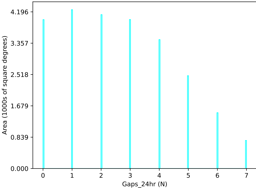
too_elab_r16_d3_griz_v3.4_10yrs u band: Gaps_24hr
