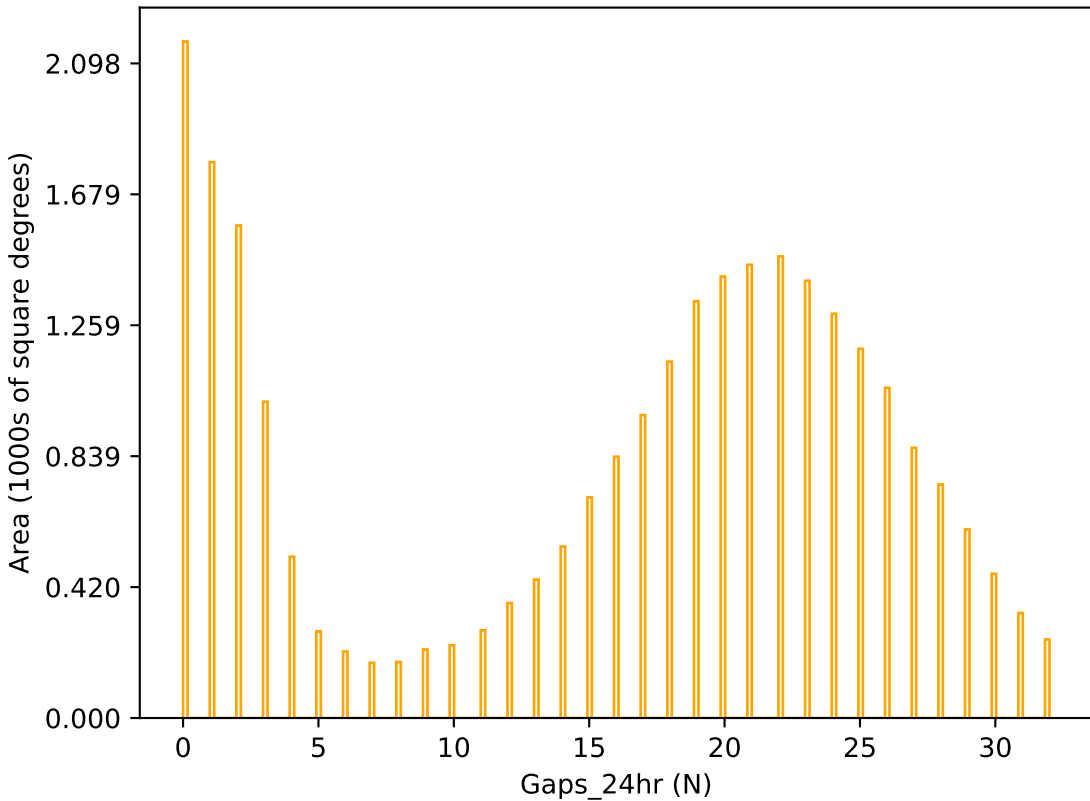
too_elab_r16_d3_griz_v3.4_10yrs r band: Gaps_24hr
