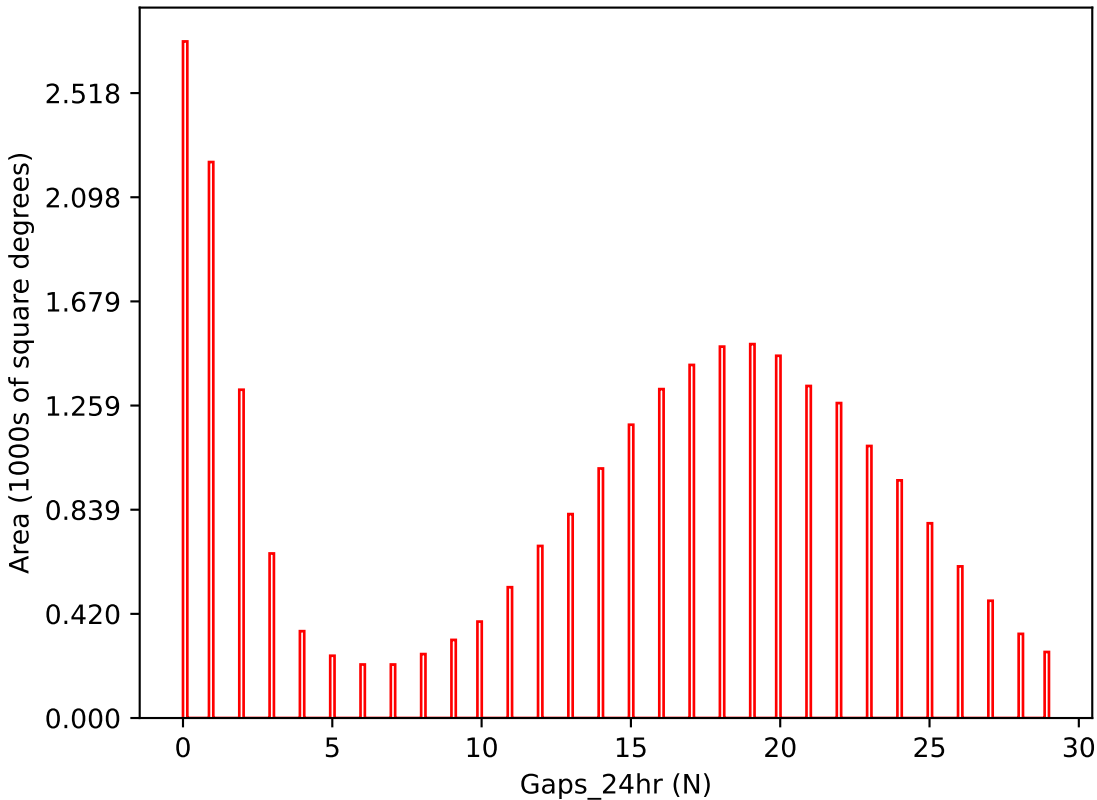
too_elab_r16_d3_griz_v3.4_10yrs i band: Gaps_24hr
