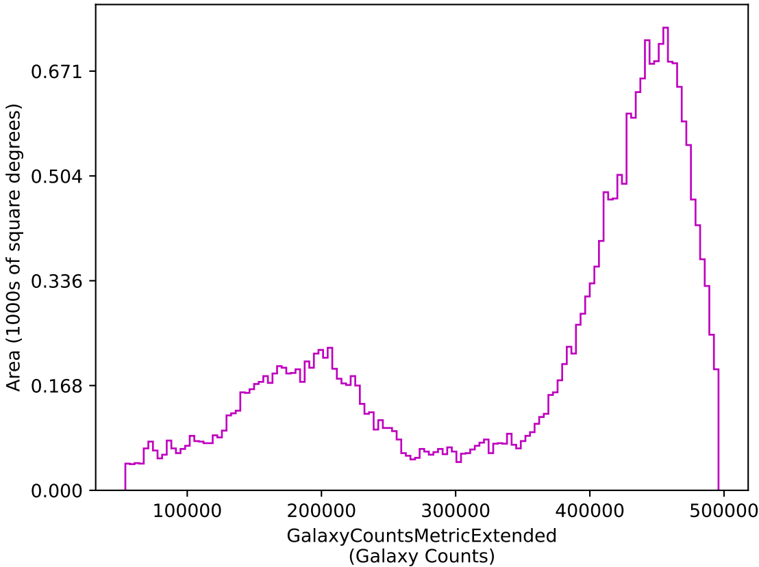
too_elab_r16_d3_griz_v3.4_10yrs z: GalaxyCountsMetricExtended
