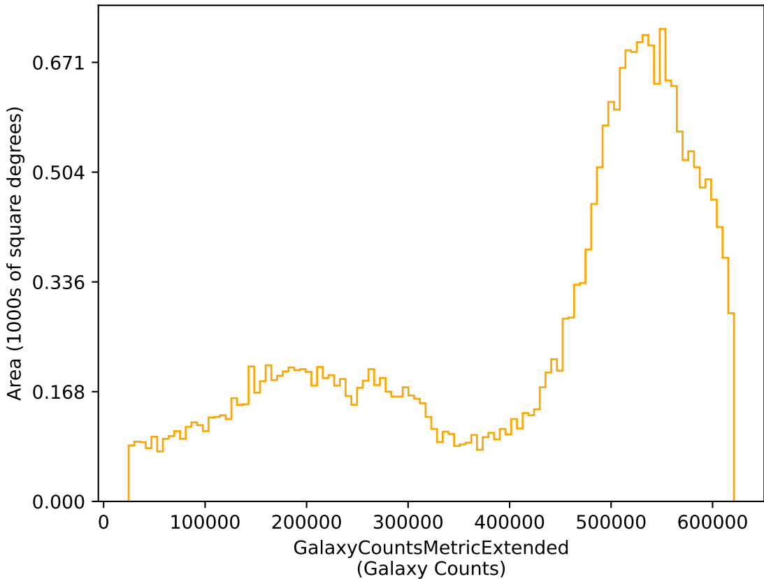
too_elab_r16_d3_griz_v3.4_10yrs r: GalaxyCountsMetricExtended
