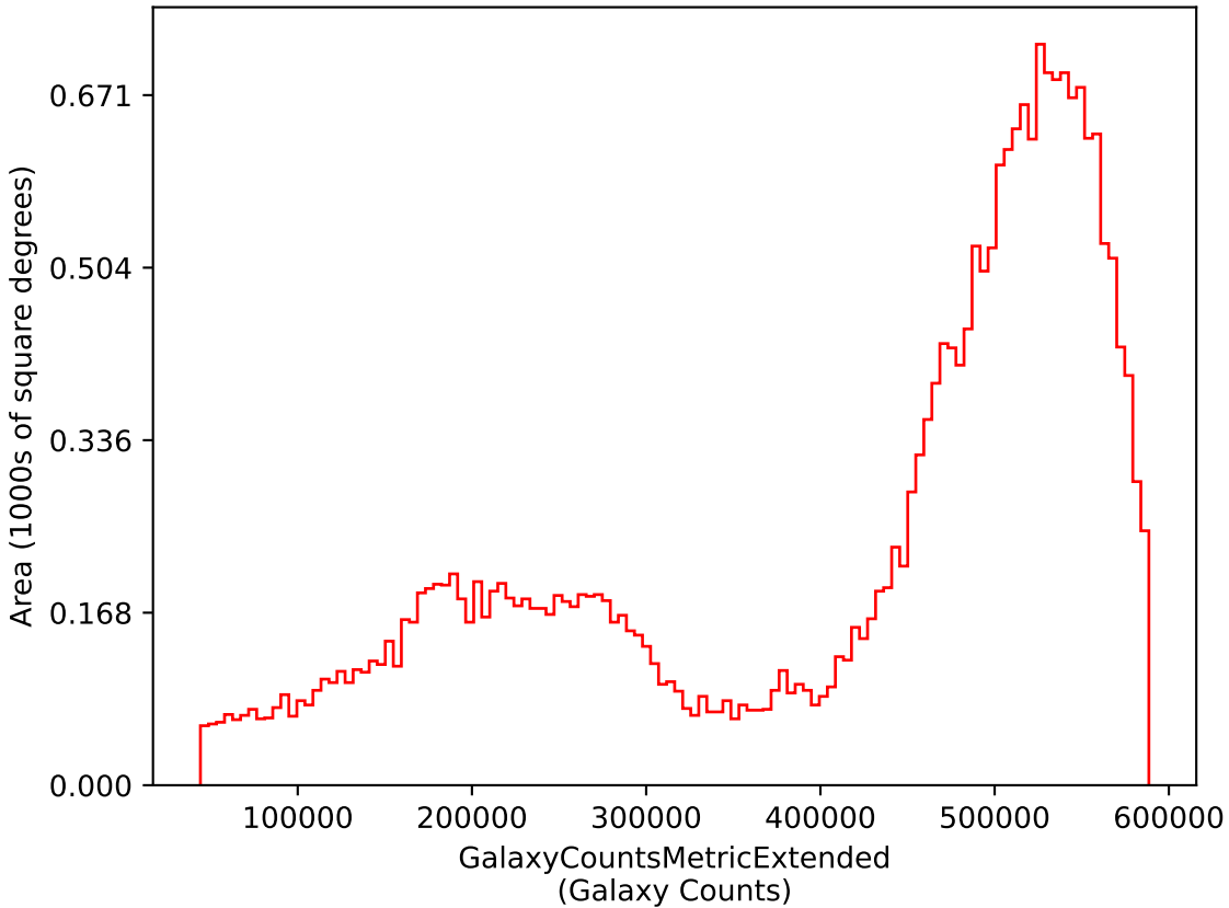
too_elab_r16_d3_griz_v3.4_10yrs i: GalaxyCountsMetricExtended
