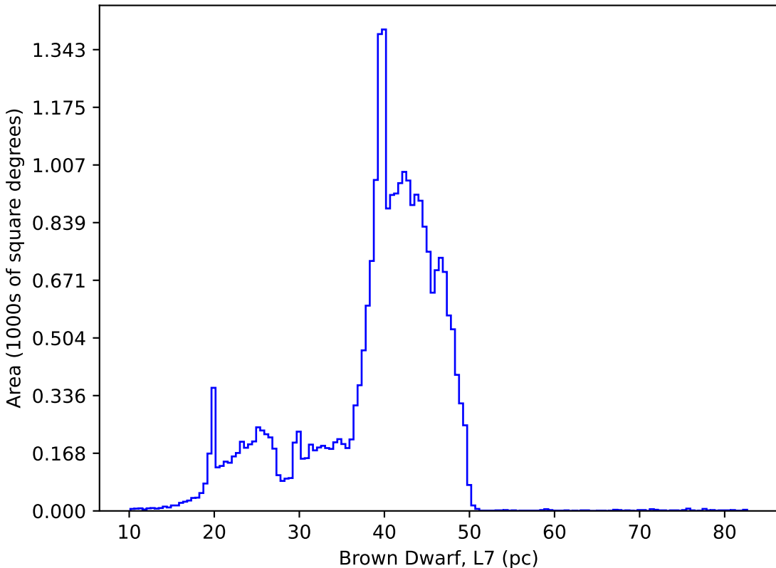
too_elab_r16_d3_griz_v3.4_10yrs : Brown Dwarf, L7
