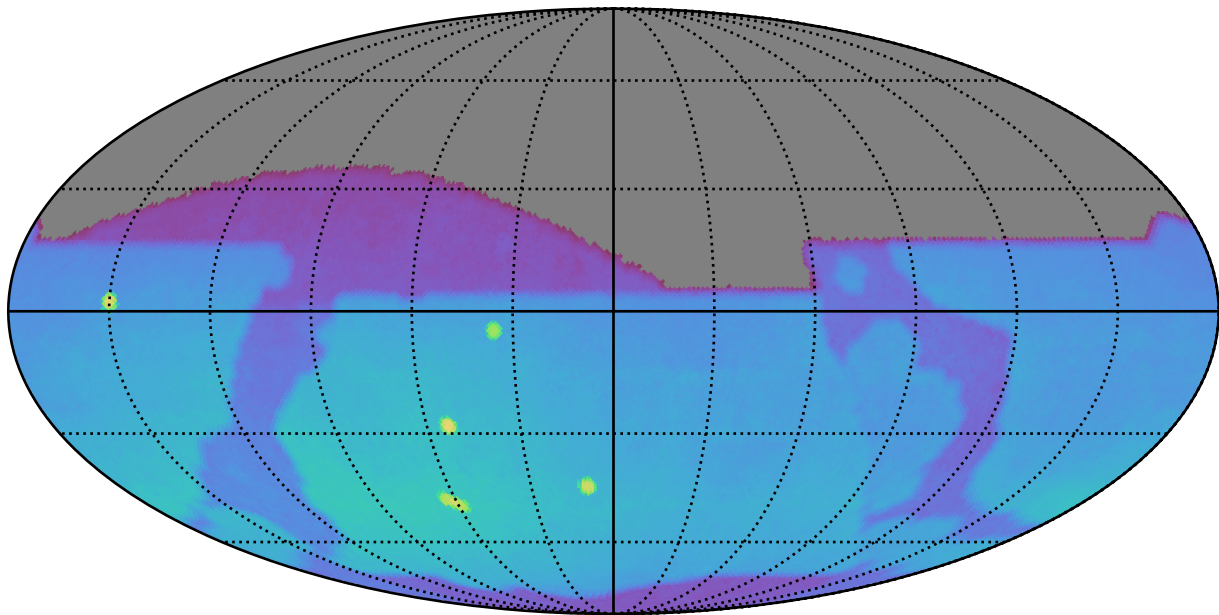
too_elab_r16_d3_griz_v3.4_10yrs : Brown Dwarf, L4
