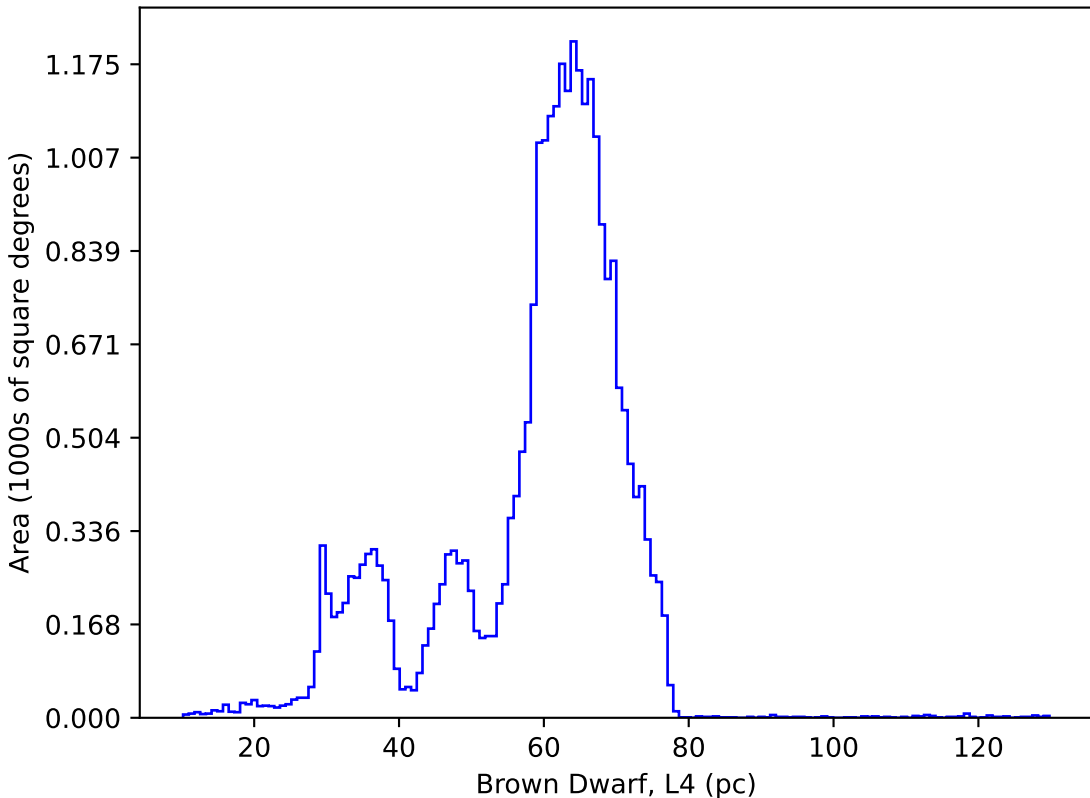
too_elab_r16_d3_griz_v3.4_10yrs : Brown Dwarf, L4
