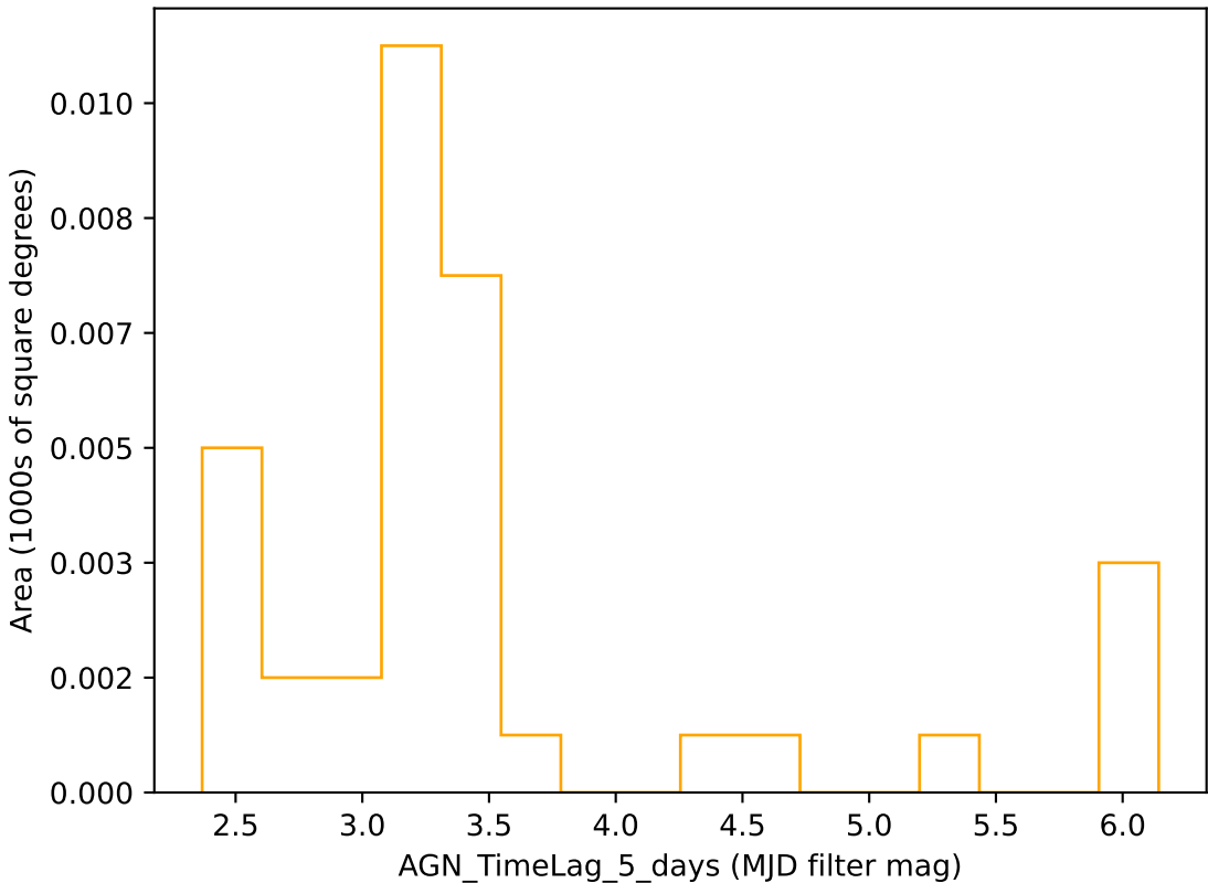
too_elab_r16_d3_griz_v3.4_10yrs r band: AGN_TimeLag_5_days
