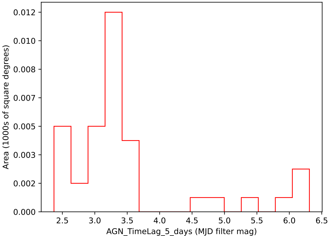
too_elab_r16_d3_griz_v3.4_10yrs i band: AGN_TimeLag_5_days
