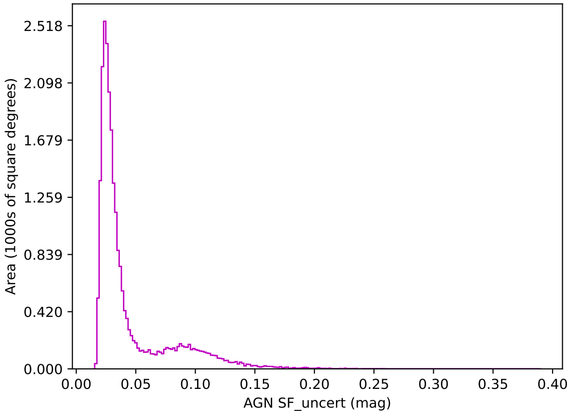
too_elab_r16_d3_griz_v3.4_10yrs z band: AGN SF_uncert
