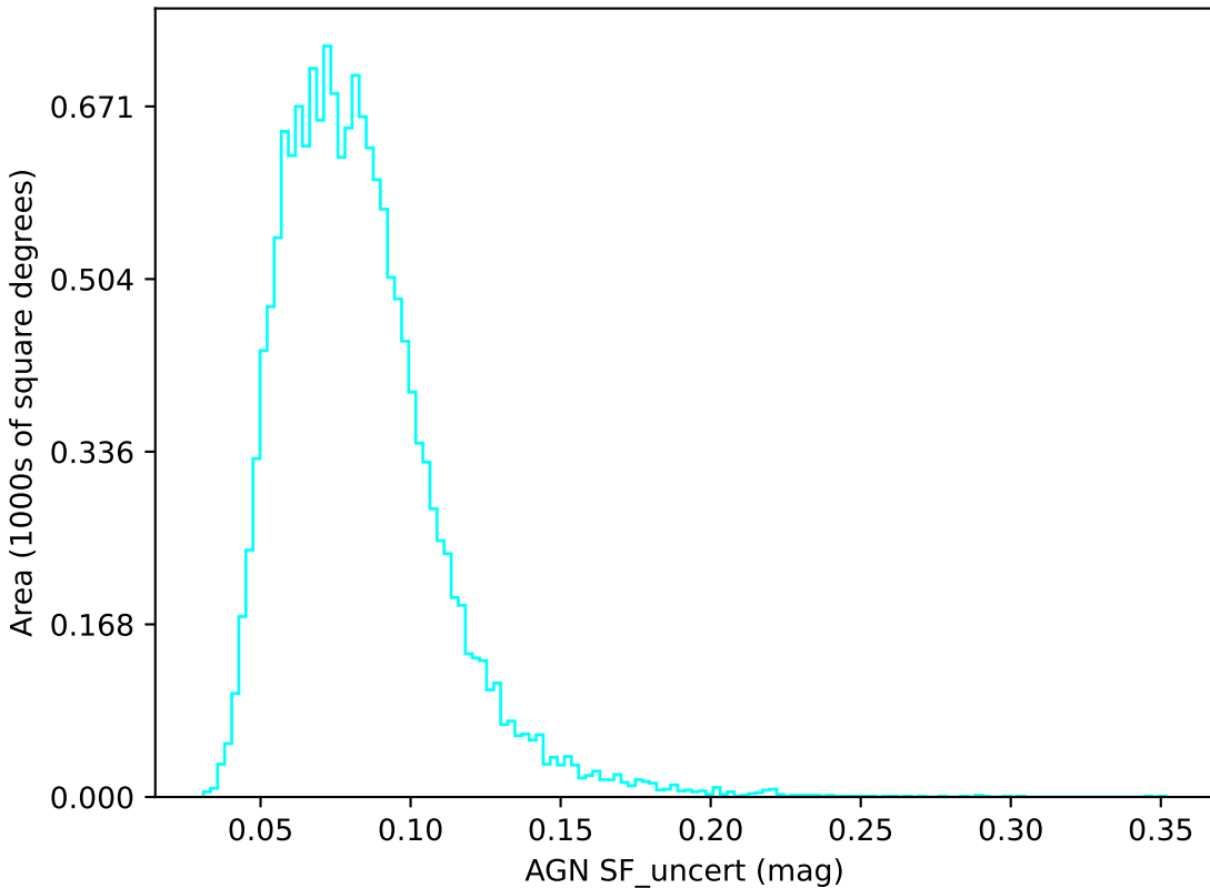
too_elab_r16_d3_griz_v3.4_10yrs u band: AGN SF_uncert
