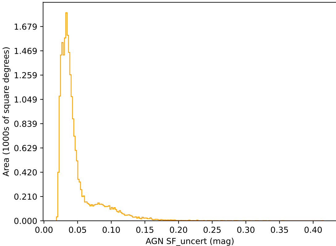
too_elab_r16_d3_griz_v3.4_10yrs r band: AGN SF_uncert
