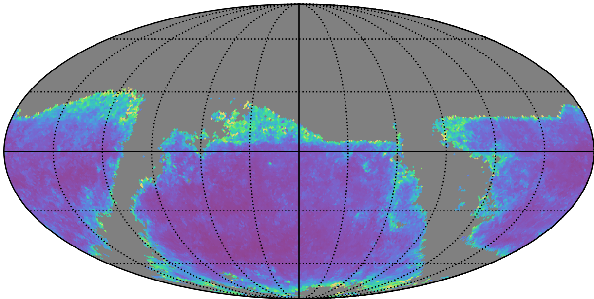
too_elab_r16_d3_griz_v3.4_10yrs g band: AGN SF_uncert
