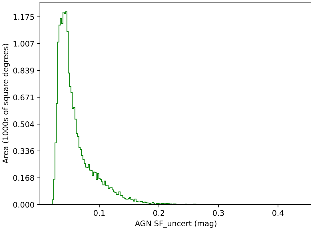
too_elab_r16_d3_griz_v3.4_10yrs g band: AGN SF_uncert
