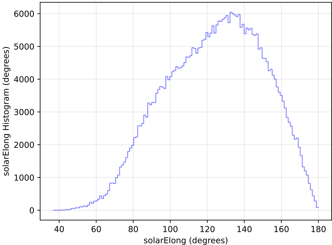
too_elab_r16_d3_griz_v3.4_10yrs WFD y band: solarElong Histogram
