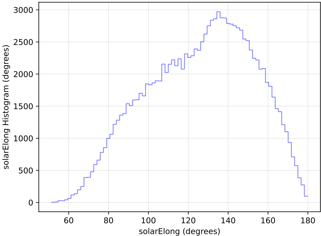
too_elab_r16_d3_griz_v3.4_10yrs WFD u band: solarElong Histogram
