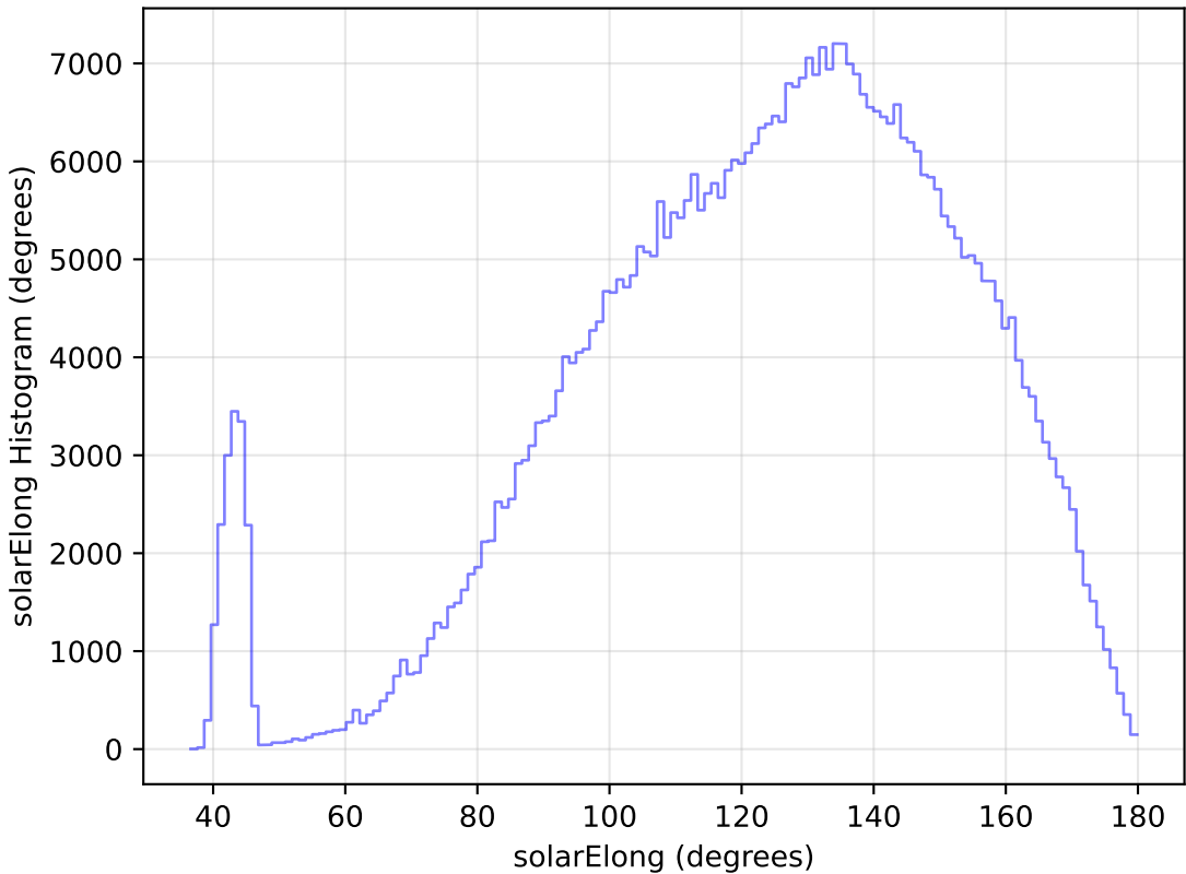
too_elab_r16_d3_griz_v3.4_10yrs WFD r band: solarElong Histogram
