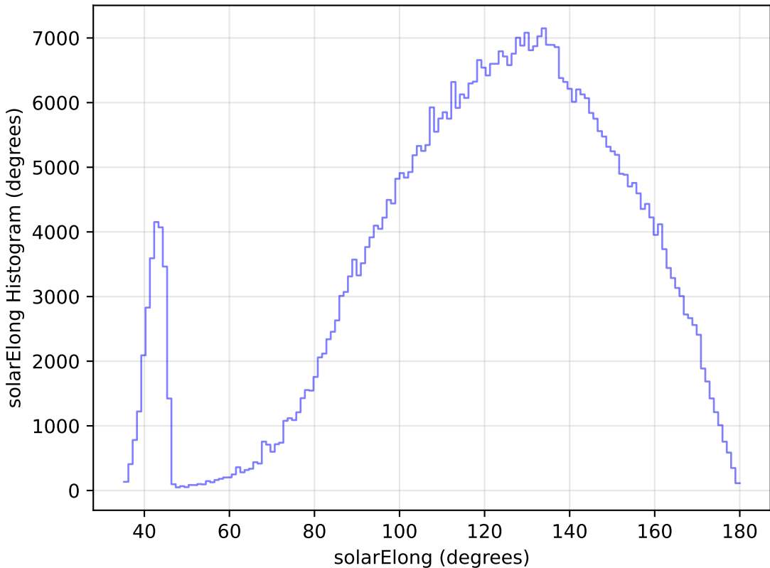
too_elab_r16_d3_griz_v3.4_10yrs WFD i band: solarElong Histogram
