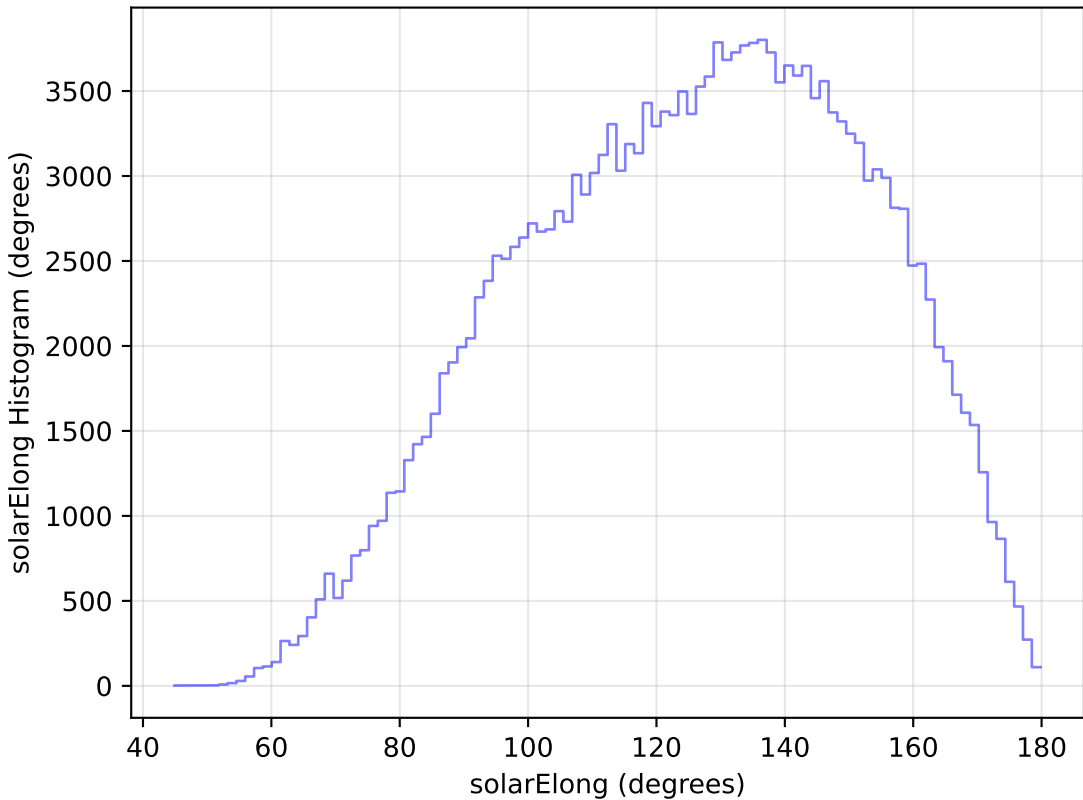
too_elab_r16_d3_griz_v3.4_10yrs WFD g band: solarElong Histogram
