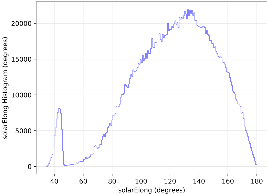
too_elab_r16_d3_griz_v3.4_10yrs WFD all bands: solarElong Histogram
