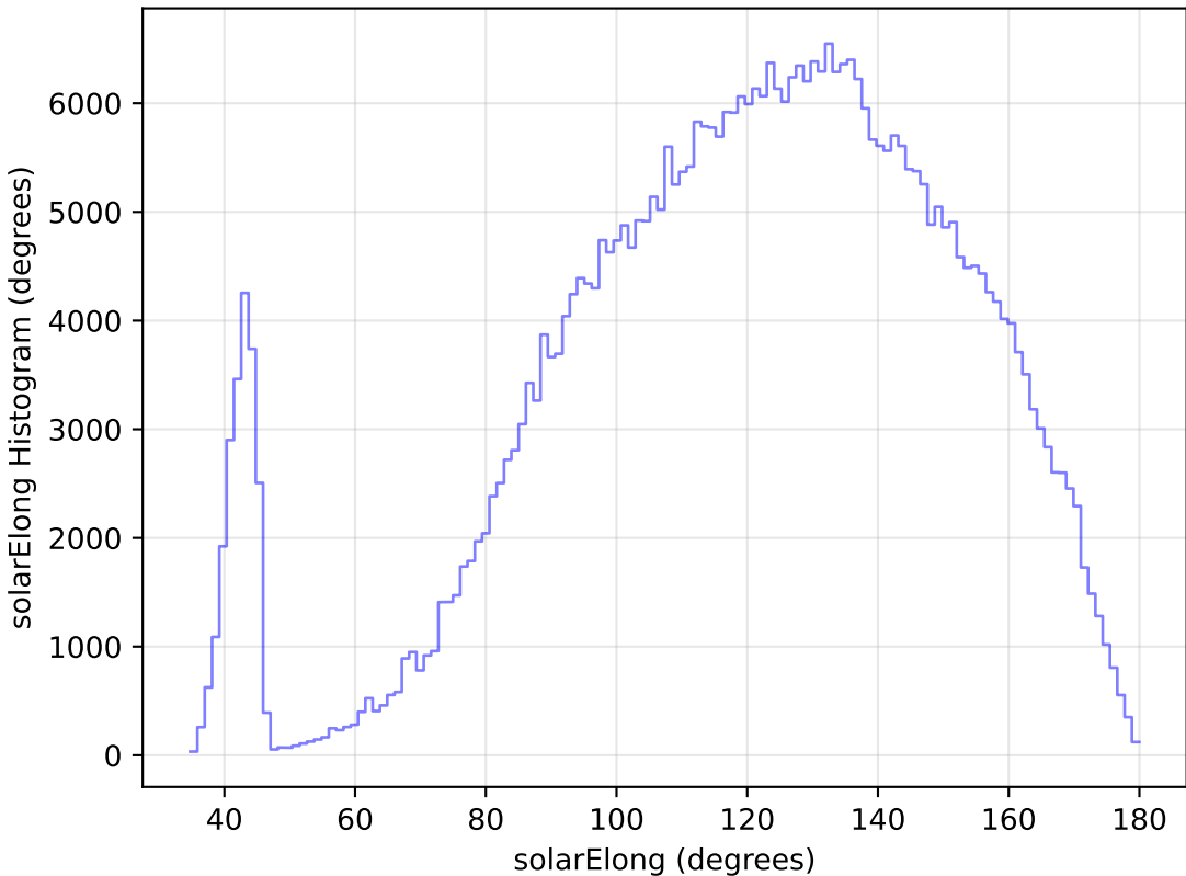
too_elab_r16_d3_griz_v3.4_10yrs All sky z band: solarElong Histogram
