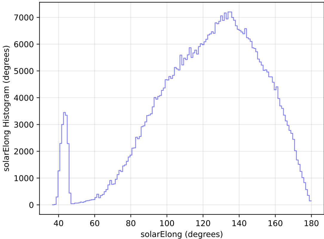
too_elab_r16_d3_griz_v3.4_10yrs All sky r band: solarElong Histogram
