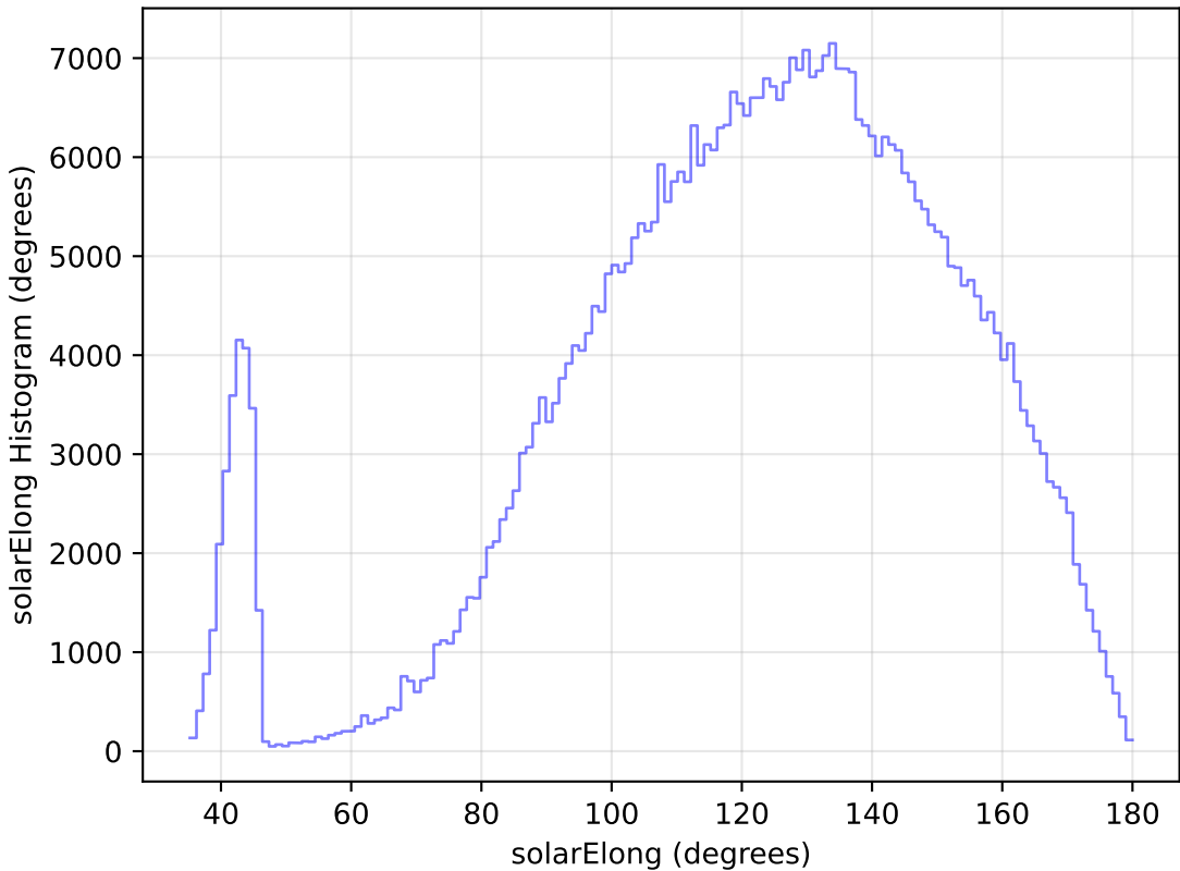
too_elab_r16_d3_griz_v3.4_10yrs All sky i band: solarElong Histogram
