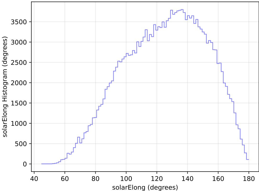
too_elab_r16_d3_griz_v3.4_10yrs All sky g band: solarElong Histogram
