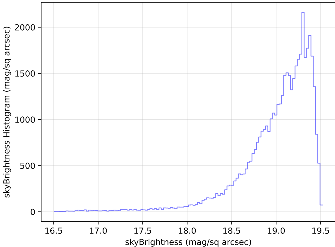
too_elab_r16_d3_griz_v3.4_10yrs Yr 1 z band: skyBrightness Histogram
