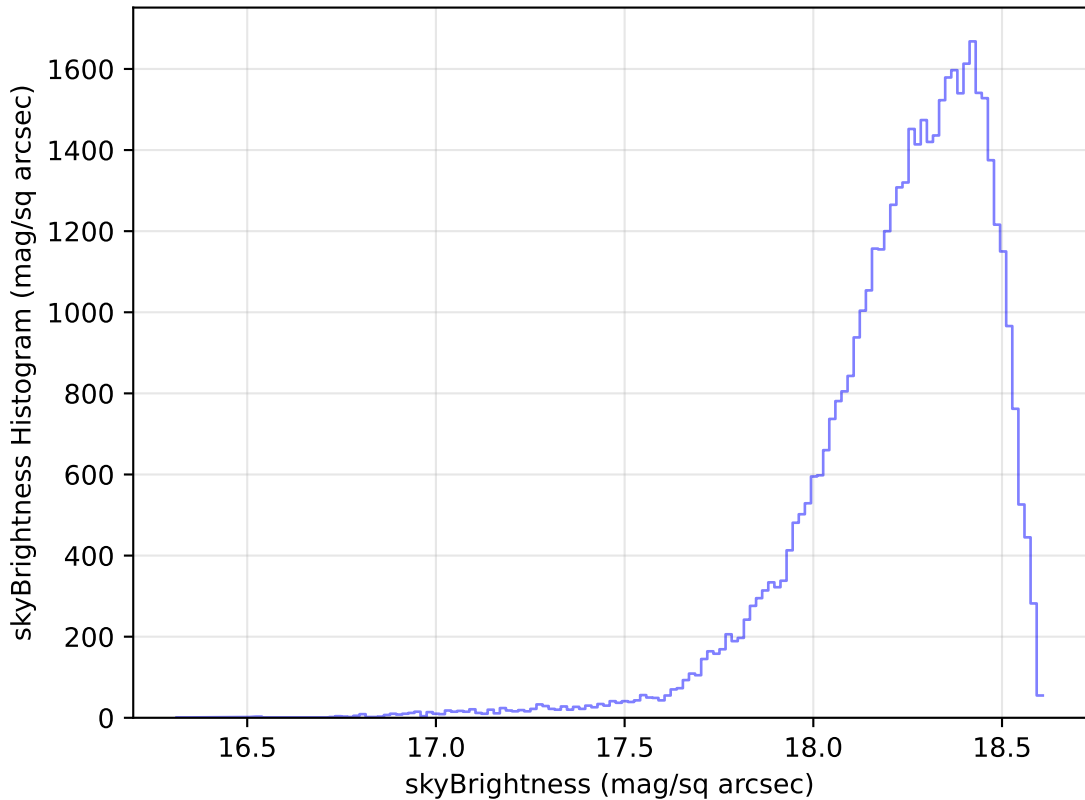
too_elab_r16_d3_griz_v3.4_10yrs Yr 1 y band: skyBrightness Histogram
